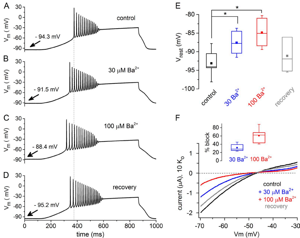
Figure 4. Maintenance of V_{\text{REST}} by inwardly rectifying \text{K}^+ channels regulates AP generation in Xenopus oocytes. Xenopus oocytes were injected with an RNA mixture of 10 ng \text{Na}_v1.4 , 2.5 ng \text{Nav}\beta1 , 2.5 ng \text{Shaker}\Delta , and 10 or 20 ng \text{K}_{\text{ir}}2.1 and incubated for 3 d before experiments. (A–E) Loose-clamp AP recordings were done using a ramp to depolarize the membrane in the absence of \text{Ba}^{2+} (2 \text{K}_0 control; A), plus 30 \mu\text{M Ba}^{2+} (B), plus 100 \mu\text{M Ba}^{2+} (C), and upon recovery from \text{Ba}^{2+} block of \text{K}_{\text{ir}} current by washout with 2 \text{K}_0 (D). The dashed, vertical line in A–D designates the approximate time of onset of the first AP in a ramp under control conditions. Arrows in A–D designate the value of V_{\text{REST}} for each recording condition. (E) Comparison of V_{\text{REST}} measured before the current ramp that elicited APs, recorded as in A–D. The impact of 30 and 100 \mu\text{M Ba}^{2+} was measured ( n = 6 ); significant differences from control values are noted by *. Box plots show 25–75% of the range (the box); the solid square inside the box is the mean V_{\text{REST}} , and the whiskers depict the maximum and minimum values. The line within the box represents the median value. (F) For the same cells as in A–E, the expression of the \text{K}_{\text{ir}}2.1 channel current was observed in TEVC recordings using a 10 \text{K}_0 solution (black trace) and a voltage ramp to elicit the \text{K}^+ currents. The current–voltage plot shows an example of block of the inward \text{K}_{\text{ir}} current by 30 \mu\text{M Ba}^{2+} (blue trace) and 100 \mu\text{M Ba}^{2+} (red trace). The recovery is in 10 \text{K}_0 (gray trace). The inset quantifies the percentage of the 10 \text{K}_0 inward current at -70 mV that was blocked by 30 or 100 \mu\text{M Ba}^{2+} ( n = 6 ).
